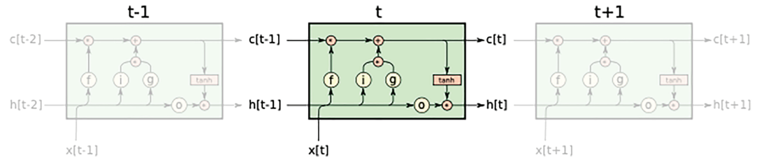
Figure 1. Visualization of (a) the standard LSTM cell as defined by equations (1)–(6).
