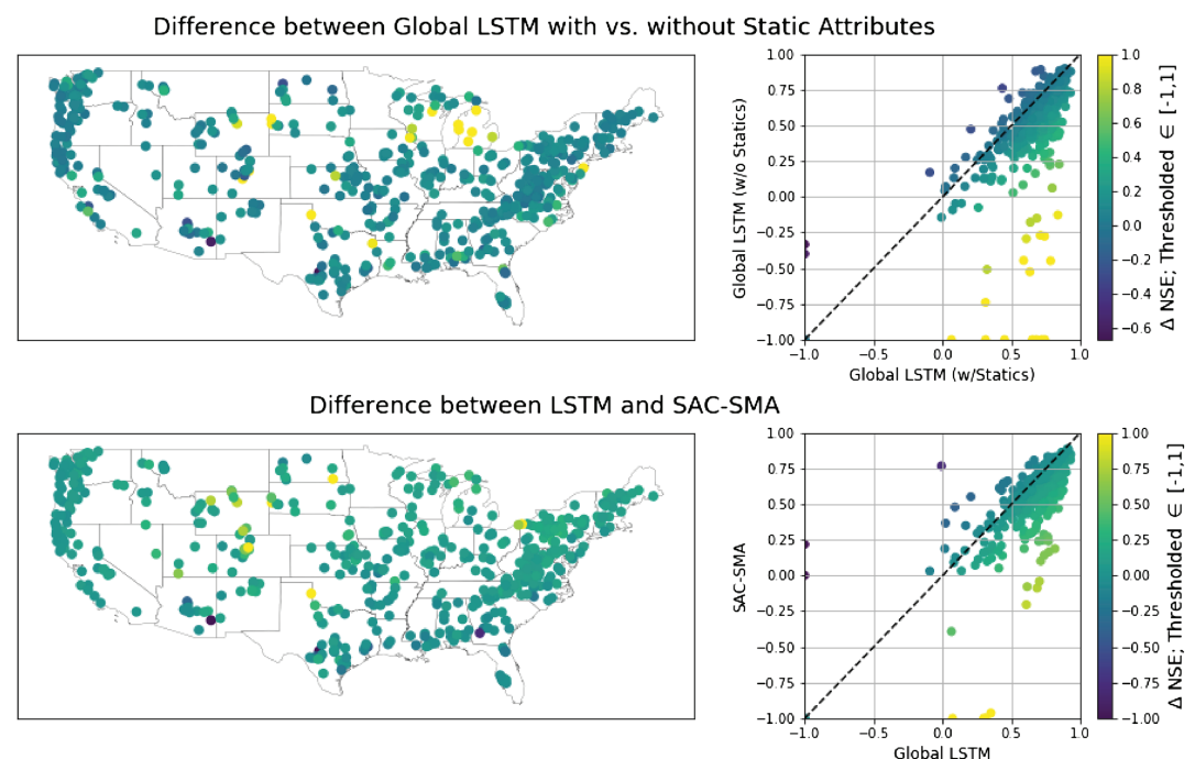
Figure 4. Comparison between the Global LSTM model with static catchment attributes and other benchmark models used in this study: (top row) LSTM without static catchment attributes and (bottom row) SAC-SMA.
