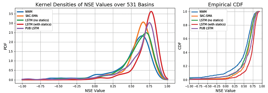
Figure 2. Frequencies of NSE values from 531 catchments given by “gauged” and “ ungauged” LSTMs, calibrated (gauged) SAC-SMA, and the National Water Model reanalysis.
