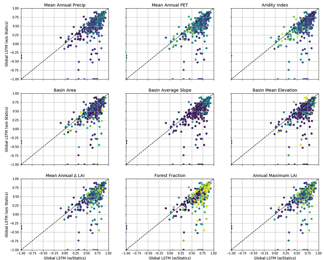
Figure 5. Scatterplots of the LSTM NSE scores in each basin with versus without static catchment attributes as model inputs. Colors indicate the relative values of a subselection of the static catchment attributes from Table 1—each subplot has a different colorscale depending on the absolute magnitudes of the specific attributes data. It is the relative values of the attributes that we care about here. There are no apparent direct relationships between the values of different catchment attributes and basins where adding catchment attribute data hurts model performance.
